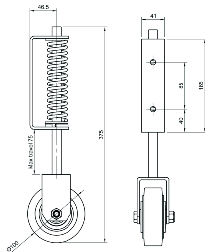
Side Elevation
